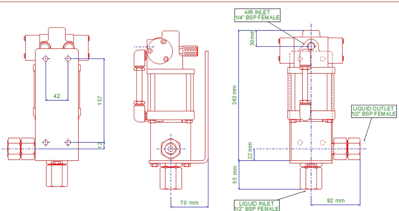
The Trojan Type 'J' Ratio 11:1, Version 'FS' With bottom inlet, and female liquid ports.
